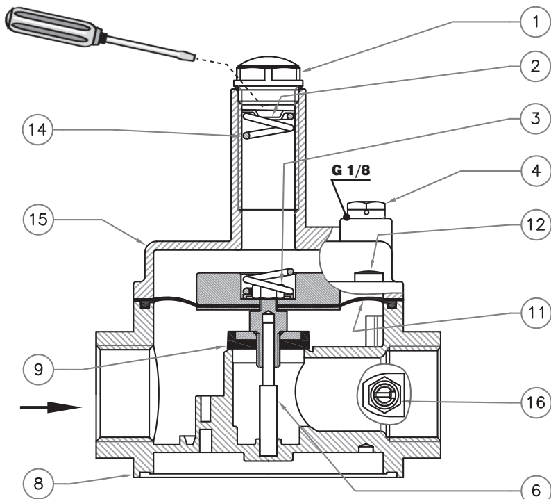
fig. 5 MVSP/1 (Compact) DN 20 - DN 25 P. max 7 bar
