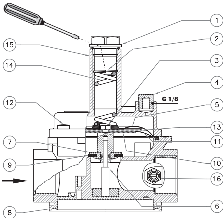
fig. 4 MVSP/1 (Compact) DN 15 - DN 20 - DN 25 P. max 1 bar
